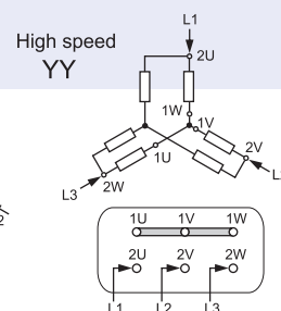
Centrifugal drive, Dahlander connection
